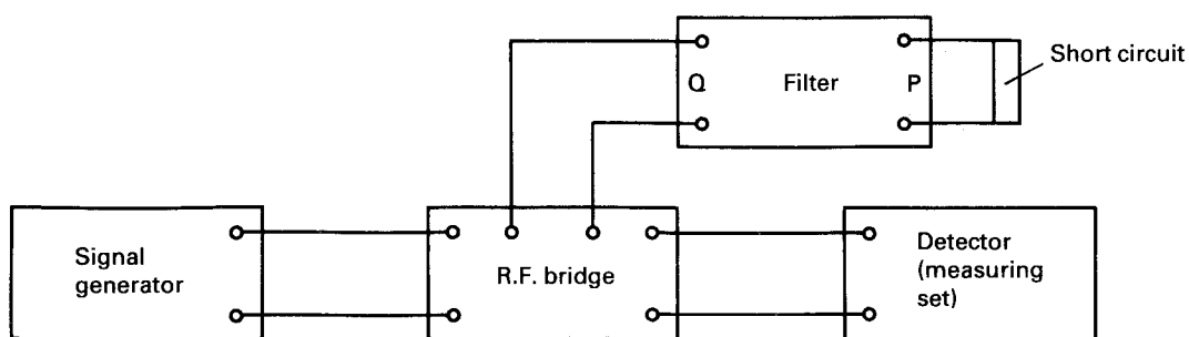
FIG. 1b. — Measurement of Thevenin impedance.
