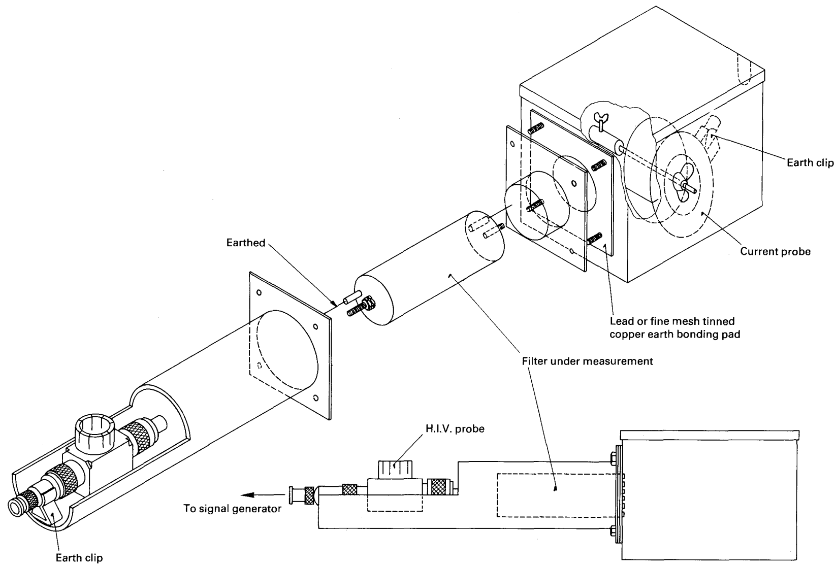
FIG. 3. — Typical method of screening for transfer impedance measurement.
